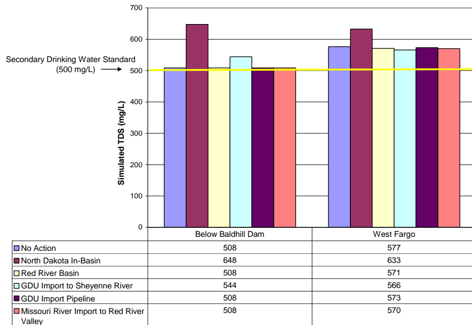
Figure 4.29 – Simulated TDS Concentrations for Unsteady Flow on the Sheyenne River.
