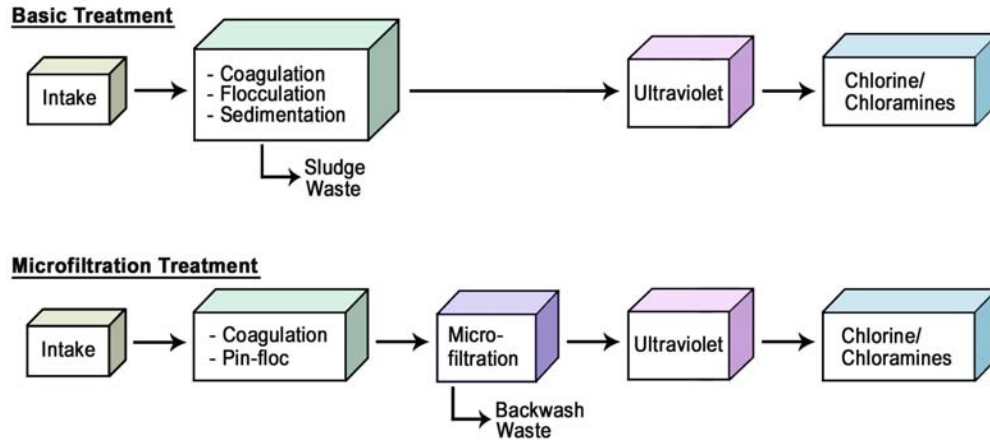
Figure 2.3 – Biota Water Treatment Processes Previously Considered in DEIS.
