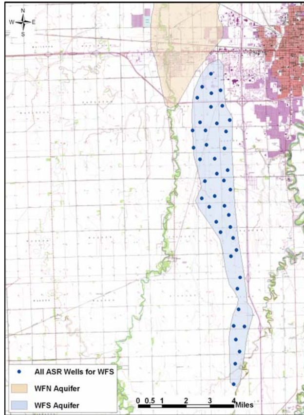
Figure 4.41 – Approximate Locations of Proposed ASR Wells in the West Fargo South Aquifer.
