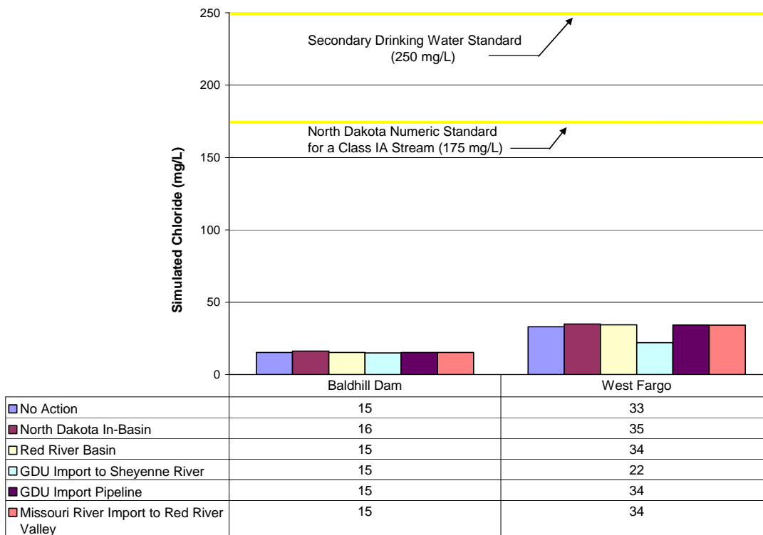
Figure 4.31 – Simulated Chloride Concentrations for Unsteady Flow on the Sheyenne River.
