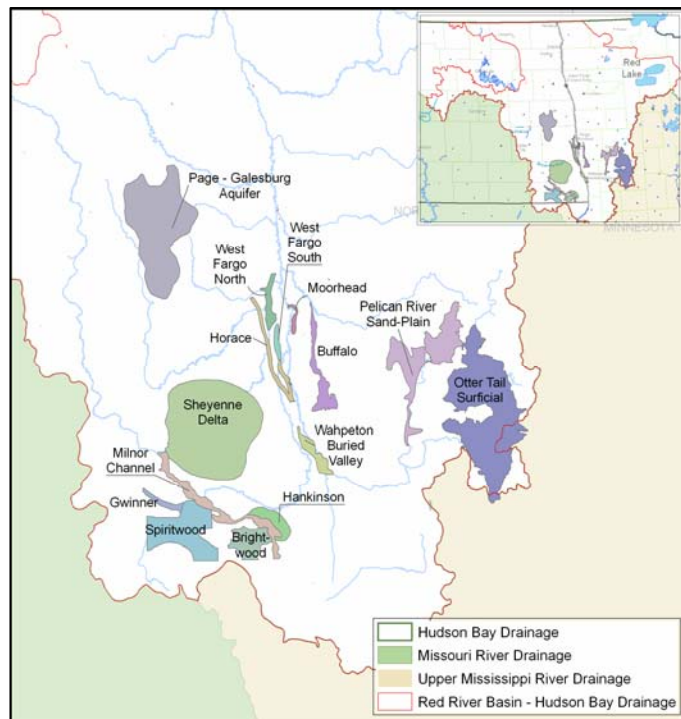
Figure 3.10 – Potentially Affected Aquifers.
