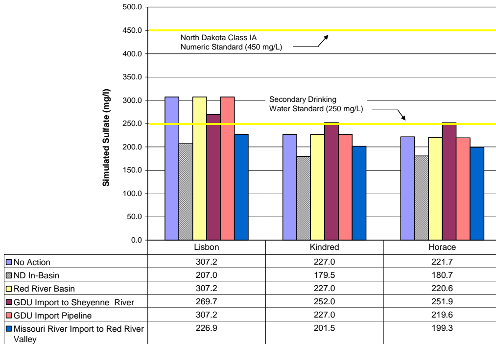
Figure 4.24 - Simulated Sulfate Concentrations for Steady Flow on the Sheyenne River.
