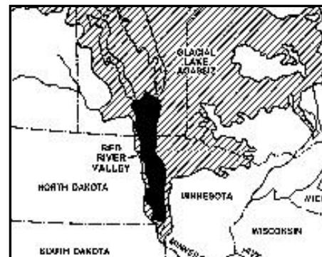
Figure 3.5 – Glacial Lake Agassiz (from Krenz and Leitch 1993)
