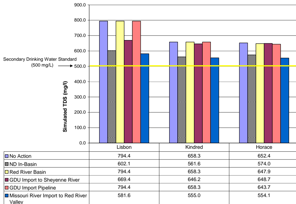
Figure 4.23 – Simulated TDS Concentrations for Steady Flow on the Sheyenne River.
