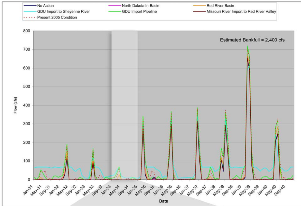
Figure 4.7 - Average Monthly Flows at Fargo, North Dakota, During a Short-term Drought 1931-1940.
