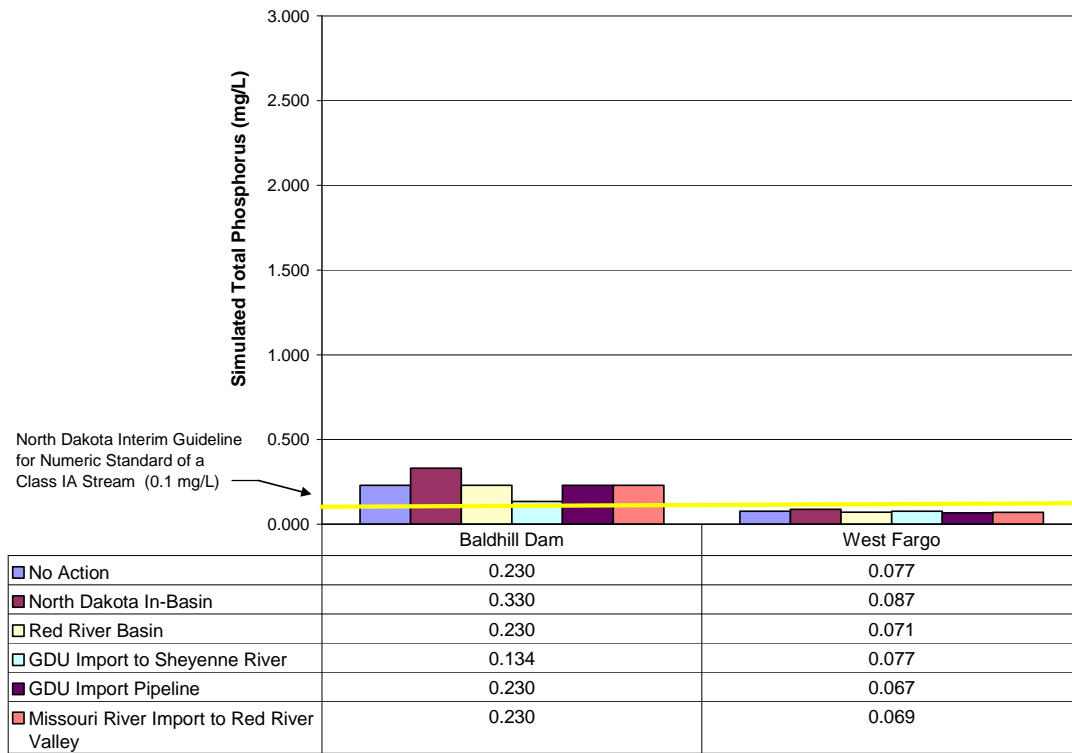
Figure 4.33 – Simulated Total Phosphorus Concentrations for Unsteady Flow on the Sheyenne River.
