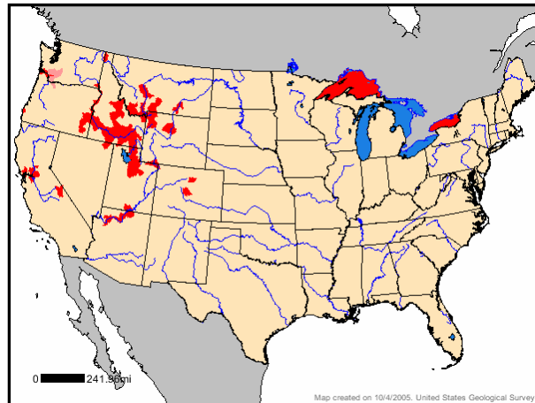
Figure 4.50 – Current Distribution of New Zealand Mudsnail in North America. Red color indicates areas with documented occurrence. Source: http://nas.er.usgs.gov/ARCIMS/interactive/interactive.asp?speciesID=1008
