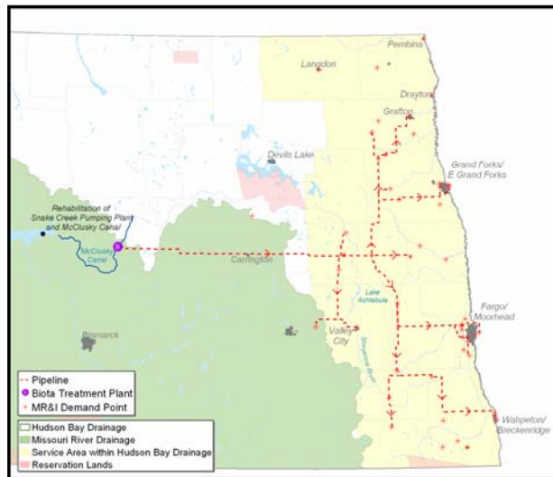
GDU Water Supply Replacement Pipeline Evaluated in the DEIS.
