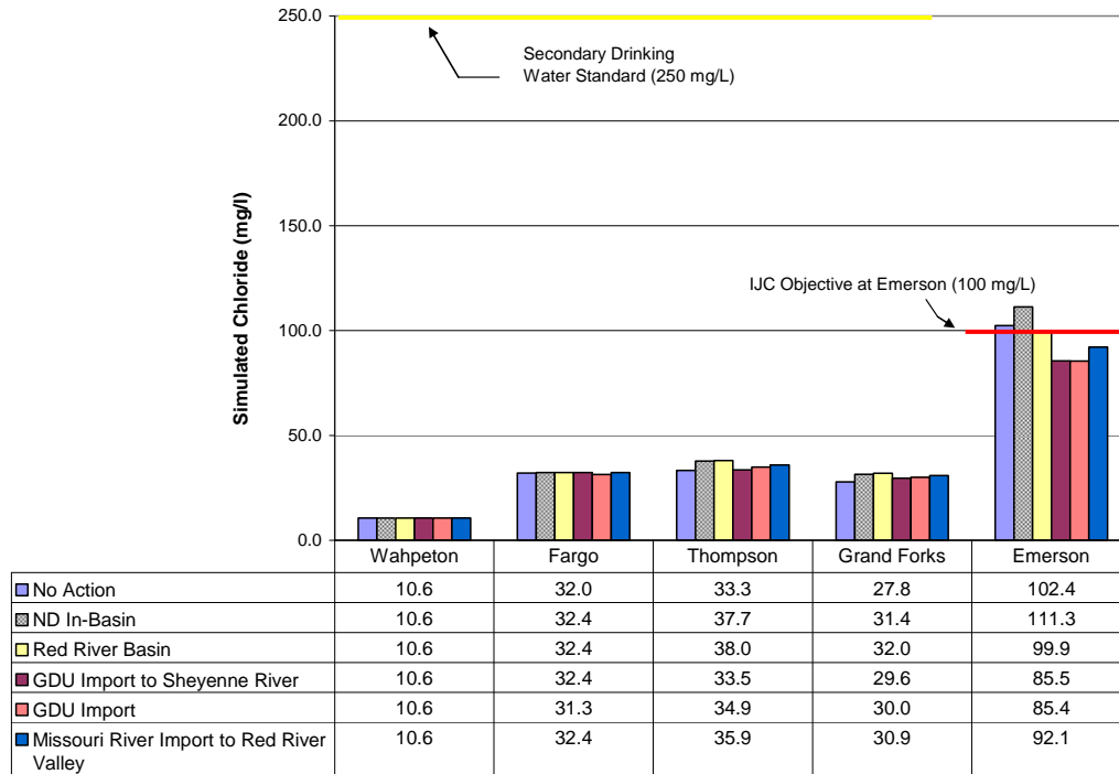
Figure 4.28 – Simulated Chloride Concentrations for Steady Flow on the Red River.
