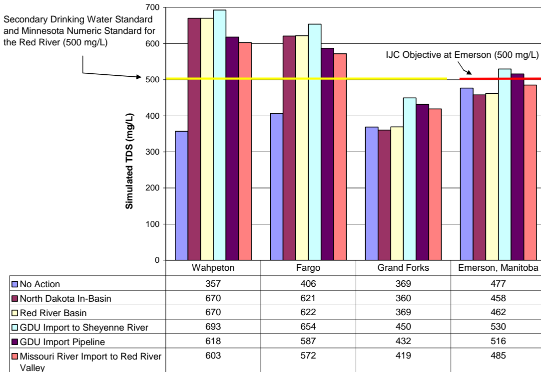
Figure 4.34 – Median TDS Concentrations for Unsteady Flow on the Red River.
