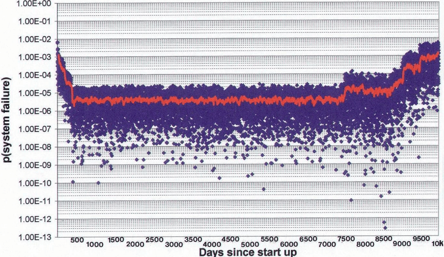
Figure 4.48 – 10,000-day Simulation of the Life-Time Distribution of Control System Failure.
