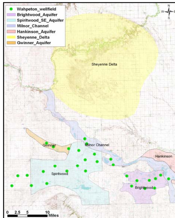
Figure 4.39 – Proposed Brightwood, Gwinner, Spiritwood, and Milnor Channel Wellfield.
