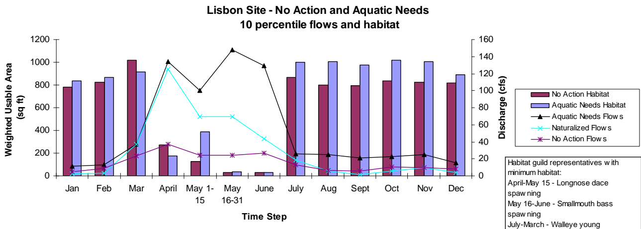
Figure 4.46 – 10 th Percentile Flow and Habitat for Representative Fish Species with Minimal Habitat from the Aquatic Needs Analysis.
