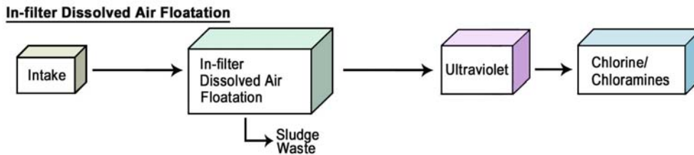
Figure 2.4 – In-filter DAF Biota Water Treatment Process Suggested by the Province of Manitoba.
