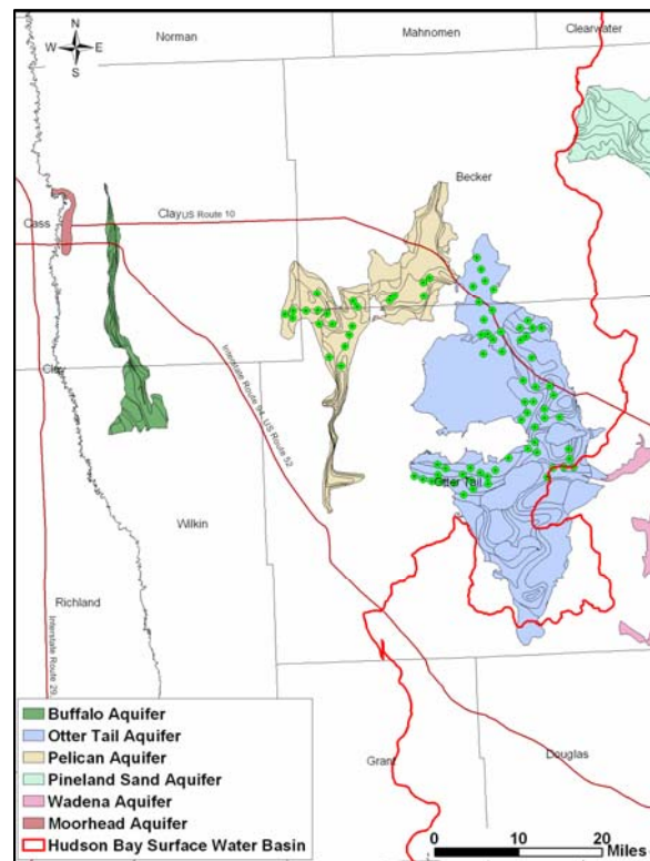
Figure 4.44 – Proposed Wellfield for Pelican River Sand-Plain and Otter Tail Surficial Aquifers.
