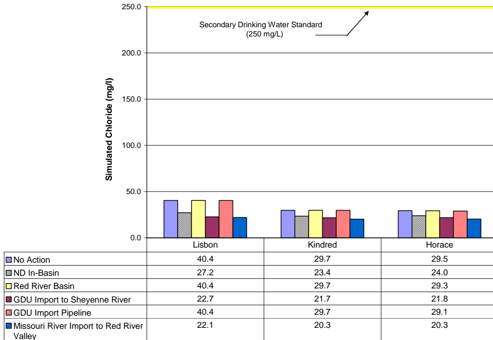
Figure 4.25 – Simulated Chloride Concentrations for Steady Flow on the Sheyenne River.
