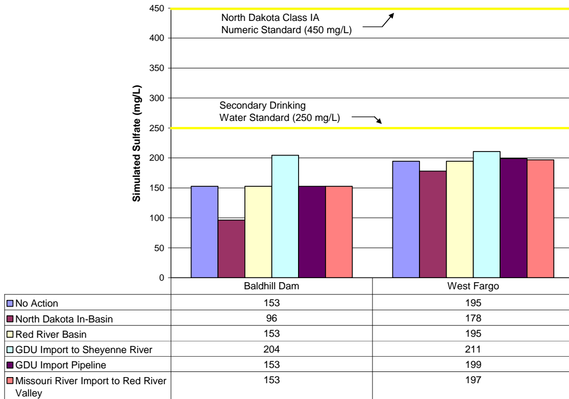
Figure 4.30 – Simulated Sulfate Concentrations for Unsteady Flow on the Sheyenne River.
