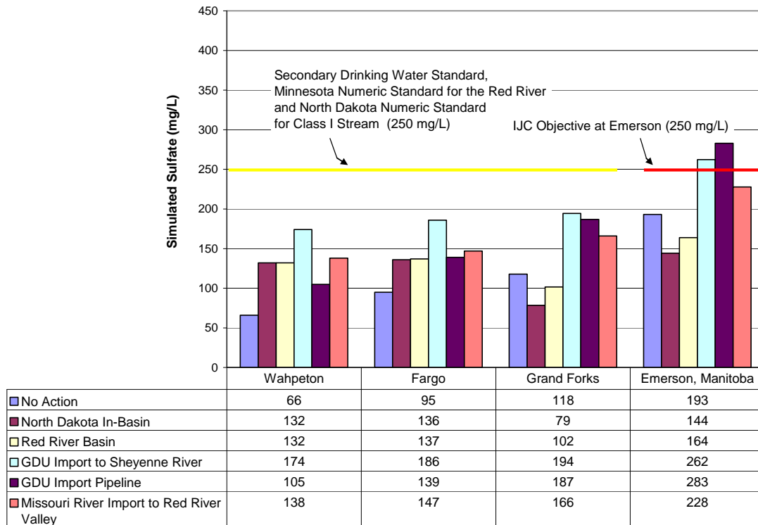
Figure 4.35 – Median Sulfate Concentrations for Unsteady Flow on the Red River.
