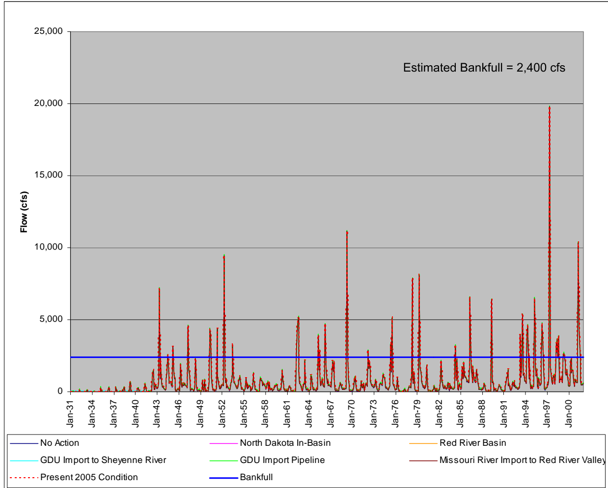
Figure 4.13 – Comparison of Average Monthly Flows on the Red River at Fargo for All Project Alternatives 1931-2001.
