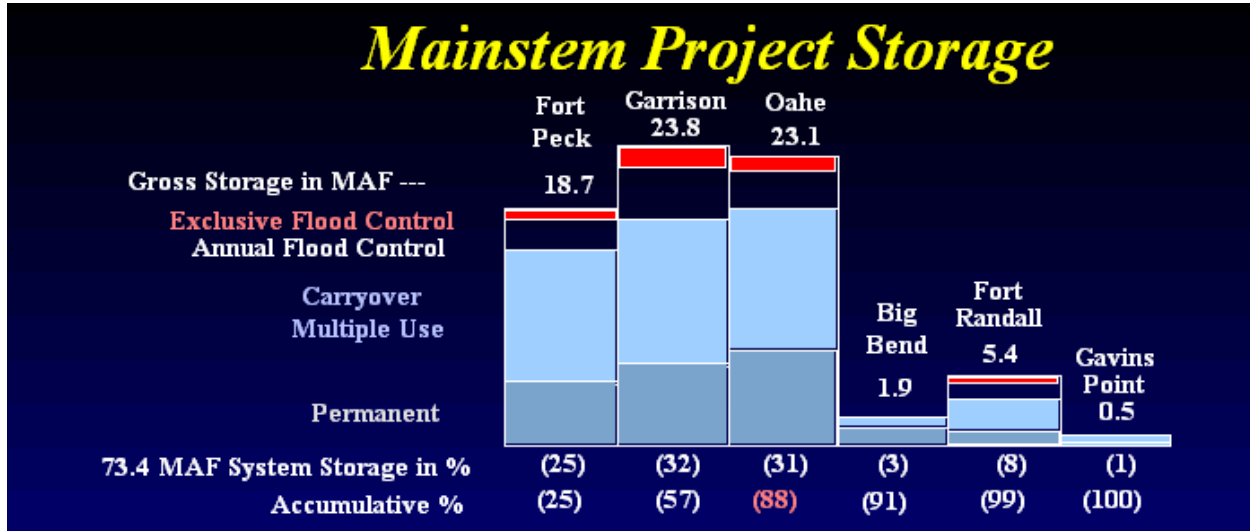
Figure 4.19 – Mainstem Project Storage (from the Reservoir Control Center, Northwestern Division, Corps of Engineers).
