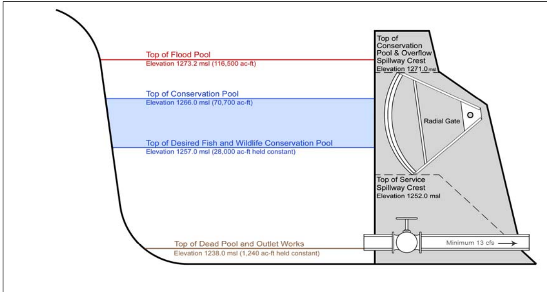
Figure 3.3 – Lake Ashtabula Pools as Defined in the Corps’ Operating Plan.
