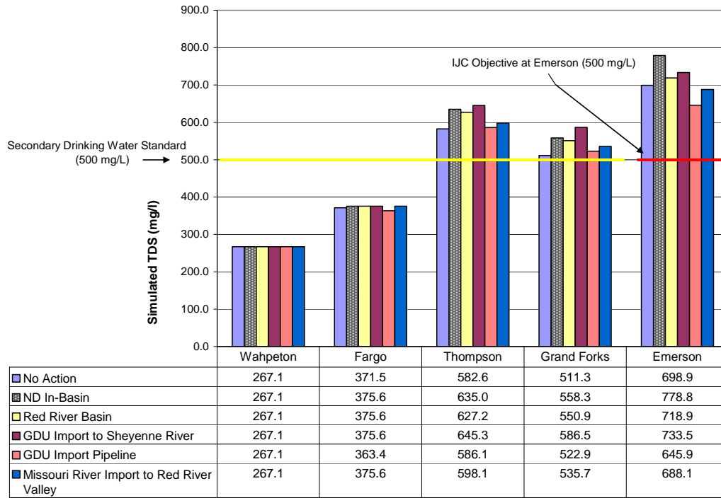
Figure 4.26 – Simulated TDS for Steady Flow on the Red River.
