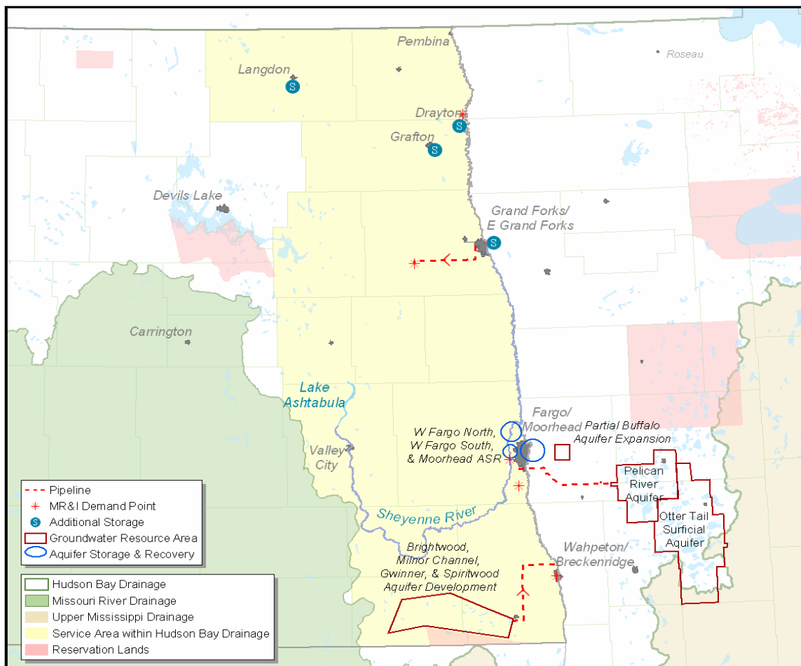
Figure 2.6 – Red River Basin Alternative.
