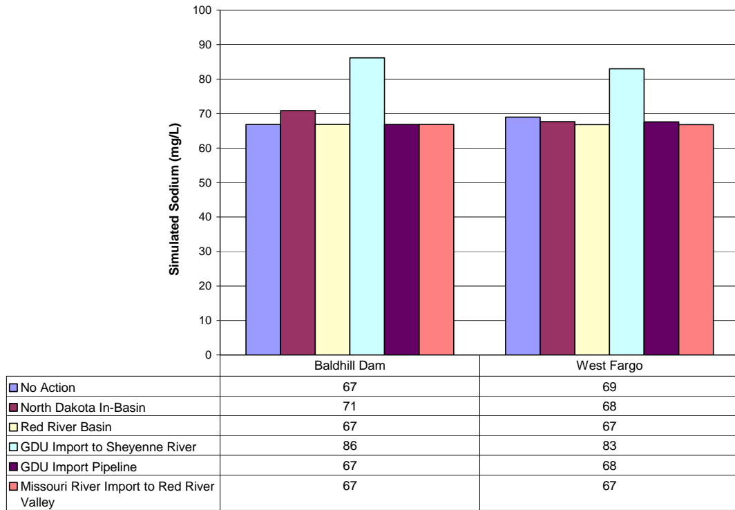
Figure 4.32 – Simulated Sodium Concentrations for Unsteady Flow on the Sheyenne River.
