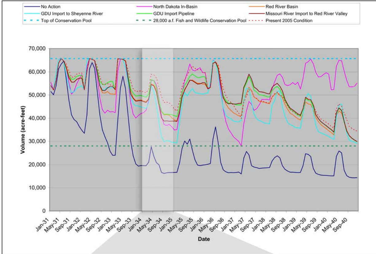
Figure 4.3 - Lake Ashtabula Average Monthly Volumes During a Drought 1931-1940.
