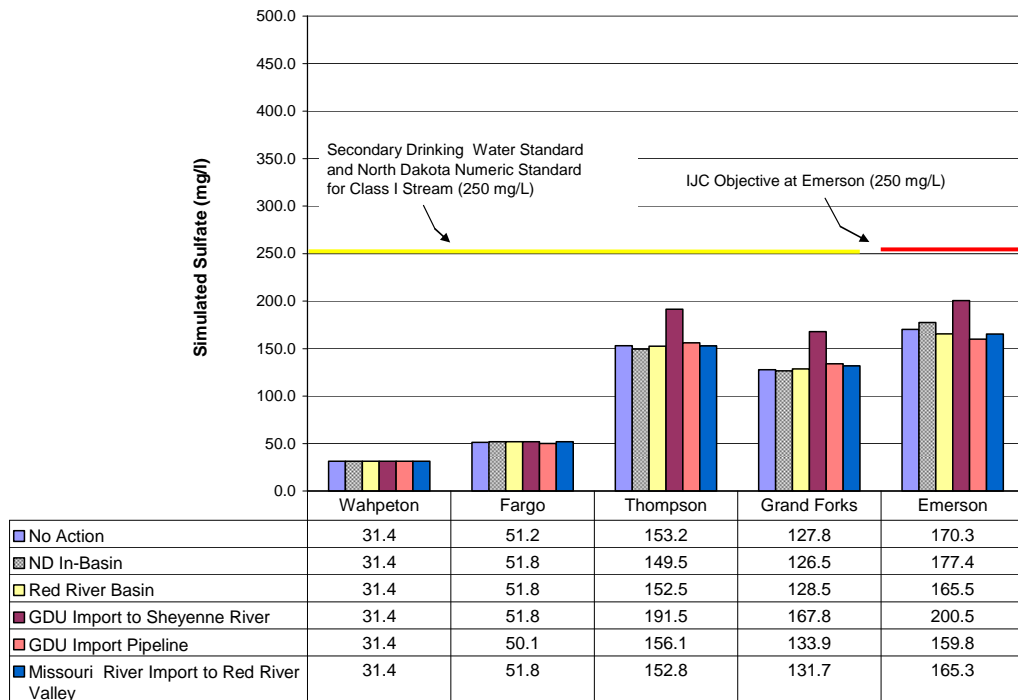
Figure 4.27 – Simulated Sulfate Concentrations for Steady Flow on the Red River.
