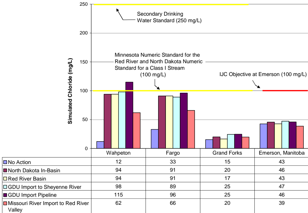
Figure 4.36 – Median Chloride Concentrations for Unsteady Flow on the Red River.
