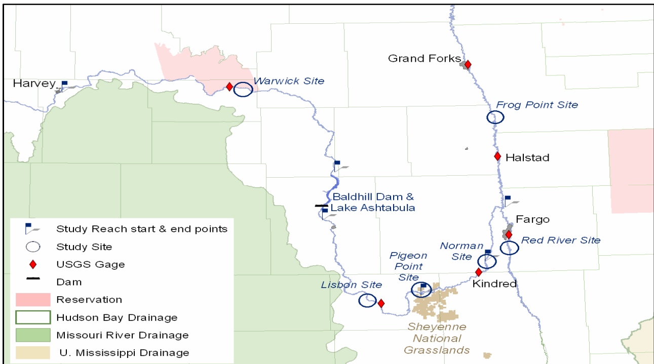
Figure 3.13 – Sheyenne River Reaches Investigated by Reclamation (2003a).
