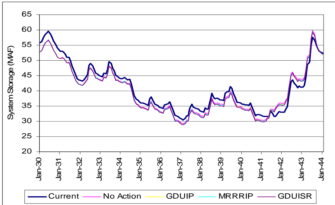
Figure 4.17 – Missouri River Basin Storage Comparison (1930-1944) (taken from Corps 2007: figure 2).
