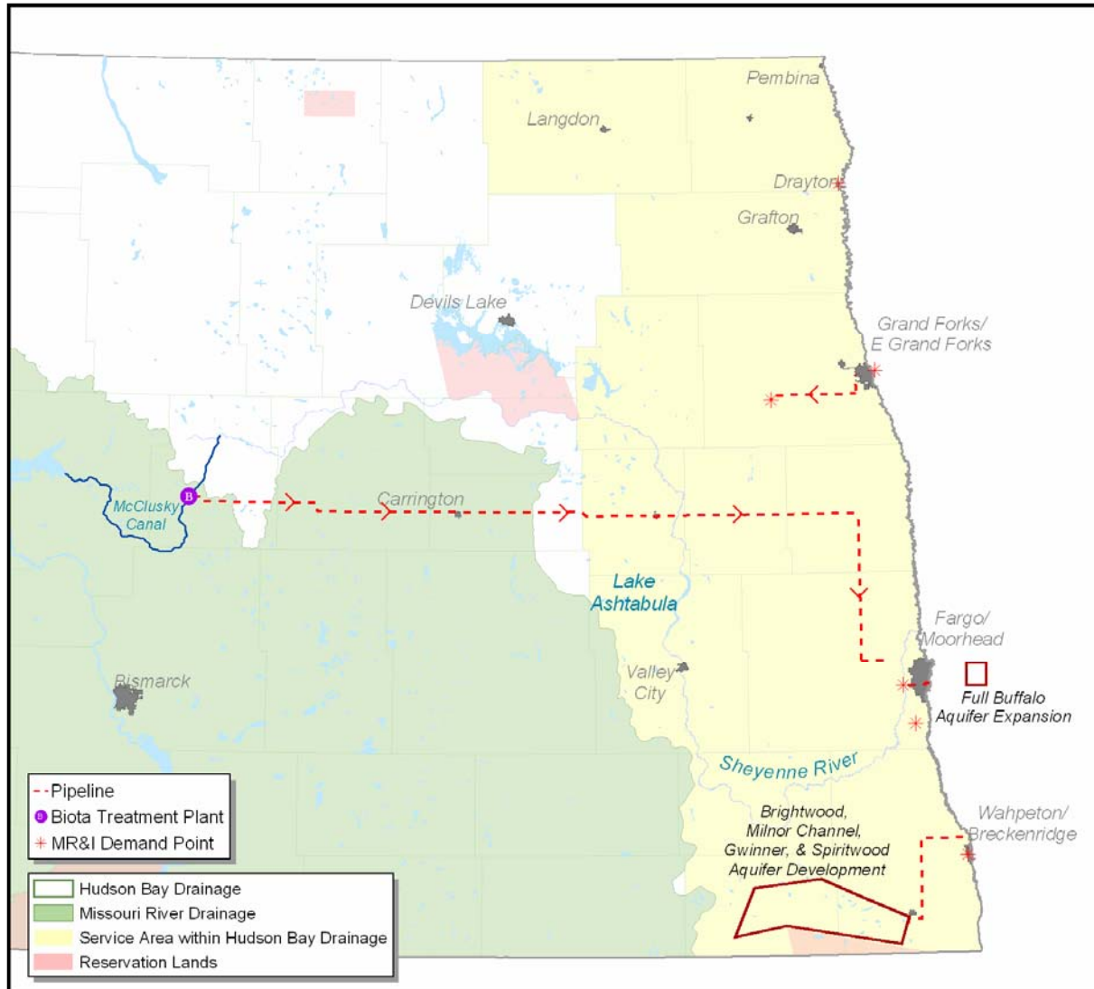
Figure 2.8 – GDU Import Pipeline Alternative.
