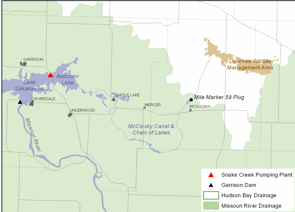
Figure 3.9 – GDU Principal Supply Works, Except for New Rockford Canal, Which is Outside the Scope of this Project.
