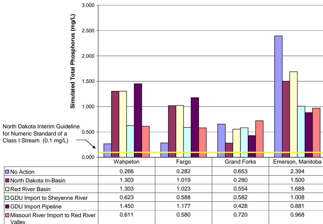
Figure 4.38 – Median Total Phosphorus Concentrations for Unsteady Flow on the Red River.
